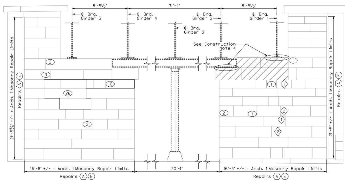
ANCHORAGE 1 - SOUTH ELEVATION
